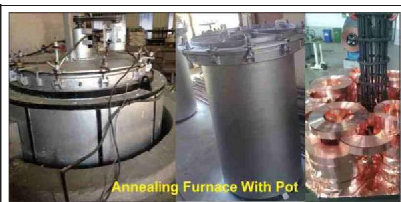
Annealing Furnace with Pot
